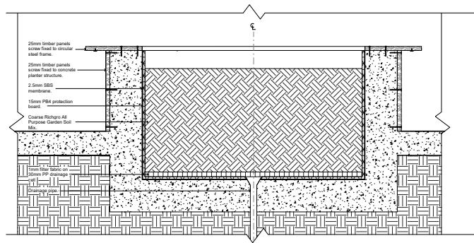
1 Planter Key Detail Section 1:10
