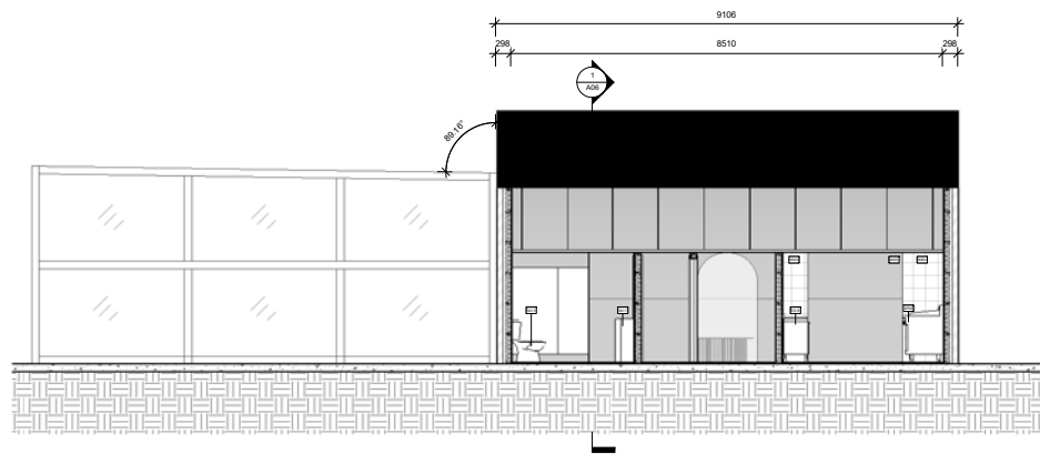
1 Section 3 1:50
