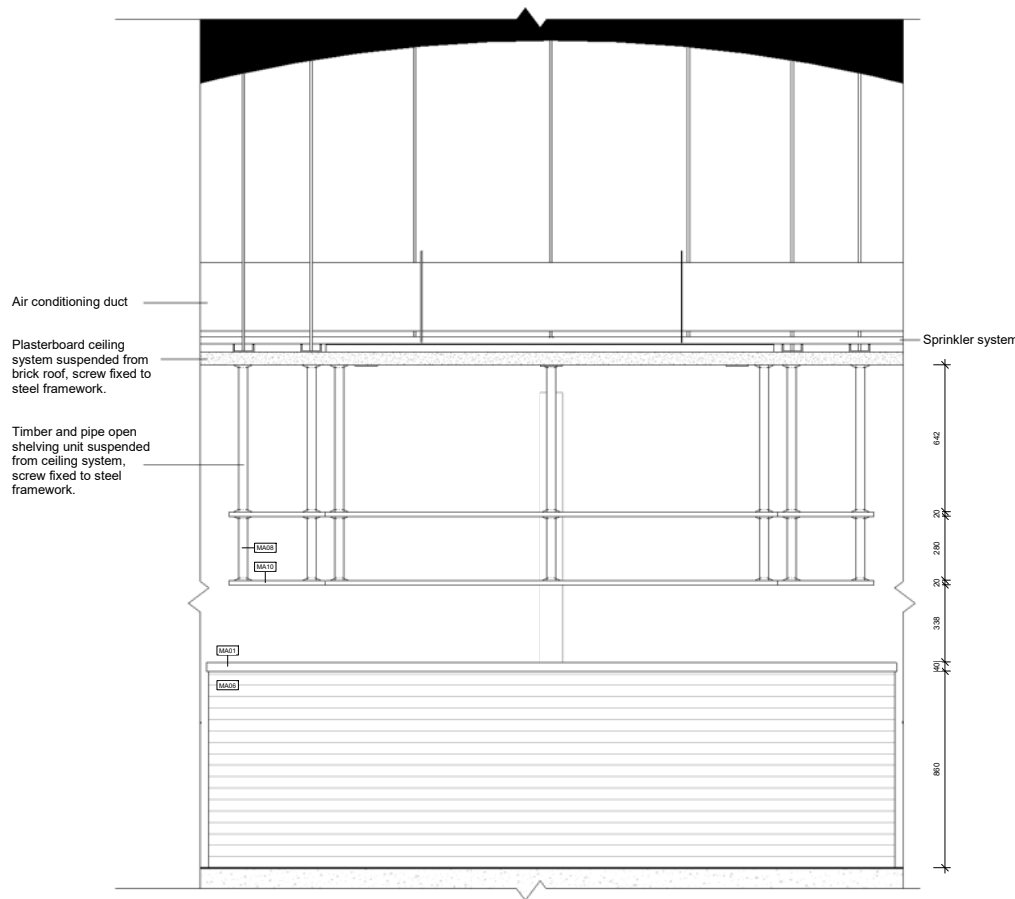
① Elevation 4 1:10
