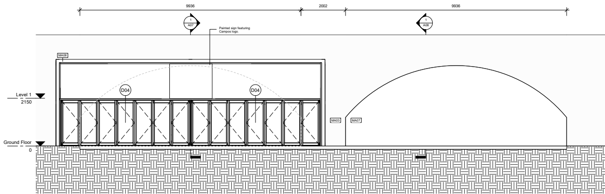
1 Shopfront South 1 : 50
