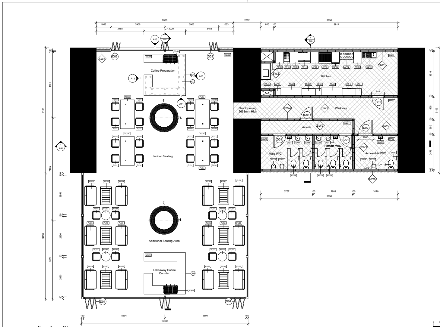
1 Furniture Plan 1 : 50
