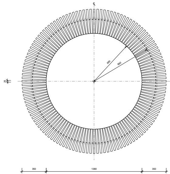
1 Planter Key Detail Plan 1 : 10
