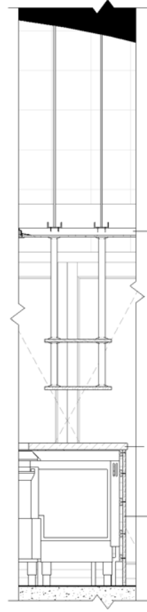
② Joinery Detail Section 2 1 : 10
